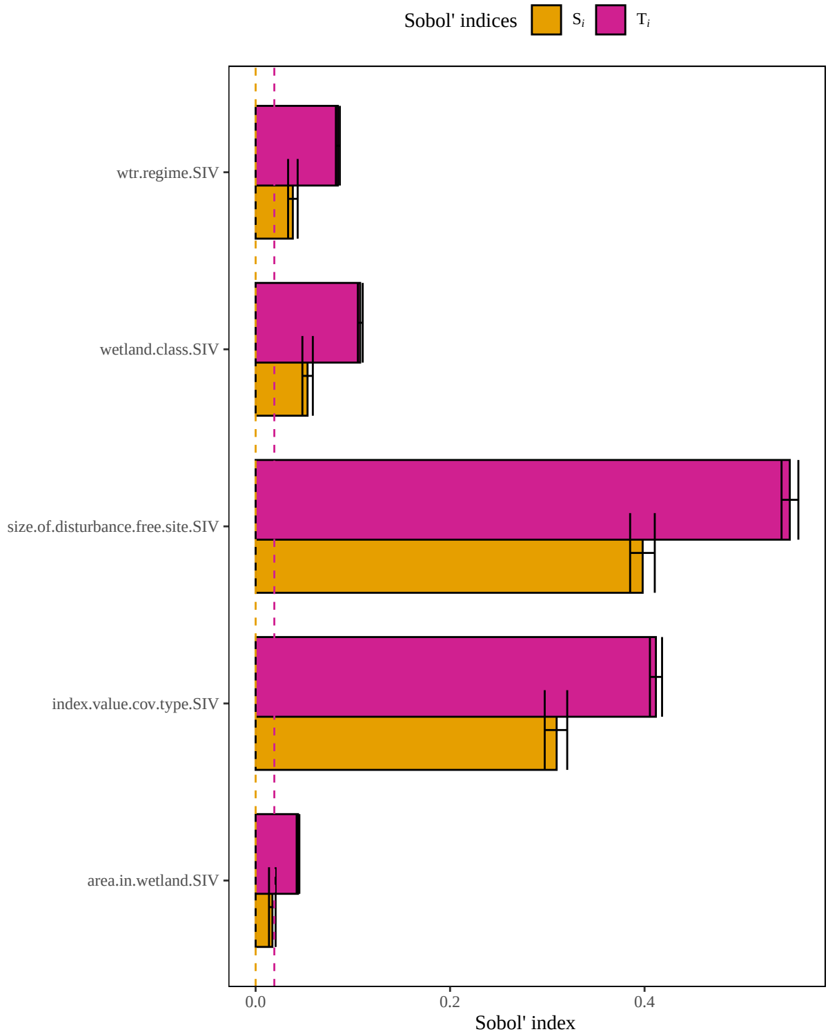
Figure 3. Results of a sensitivity analysis for the greatersandhillcrane Lt200ha model based on the original author-specified model outlined in Armbruster (1987). Dashed lines represent baseline numerical approximation error for S_i and T_i ( i.e. , dummy variables).
